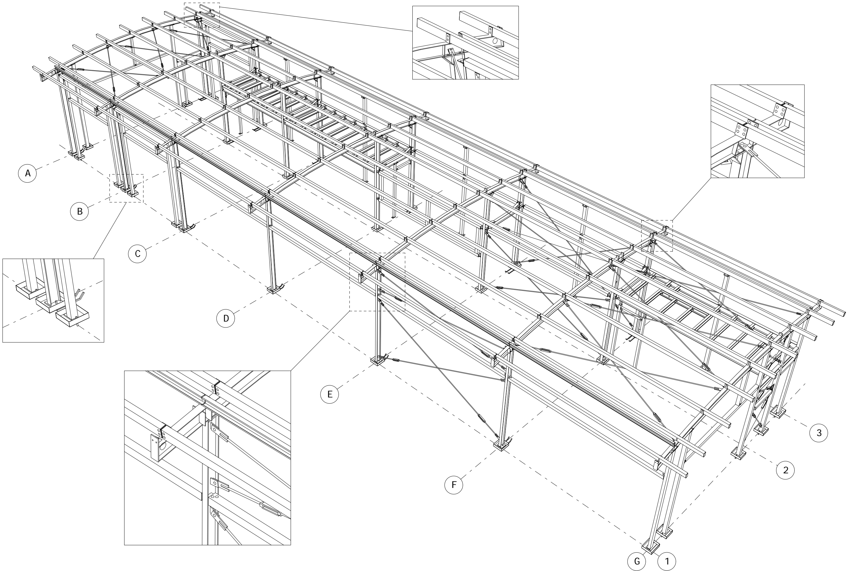
3-D VIEW
